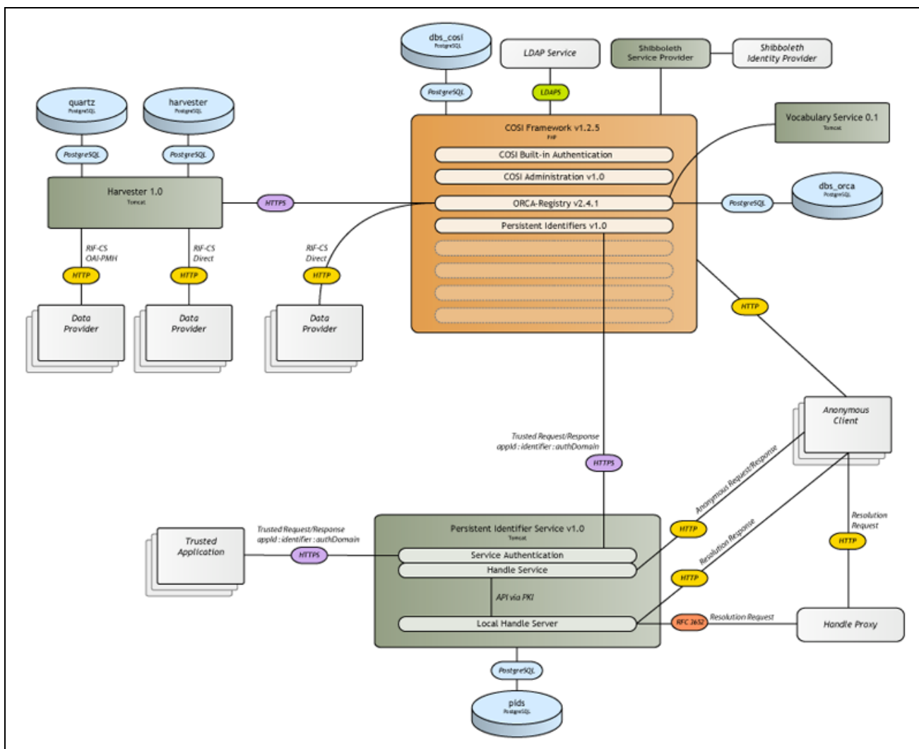
Figure 1: The COSI-Framework in context.
